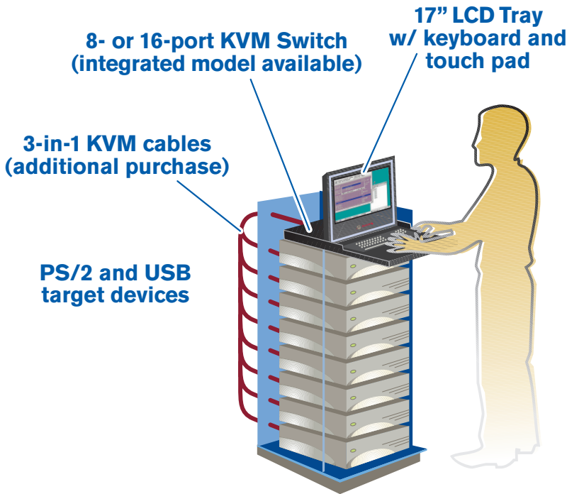
At-the-rack access using the Avocent LCD console tray with integrated KVM
